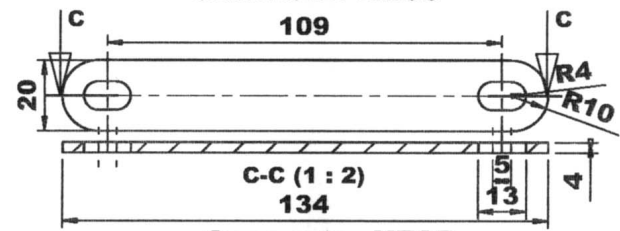
Connector HZ07
